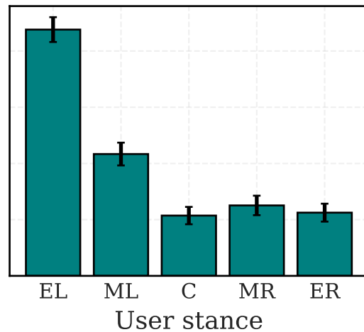
Climate
